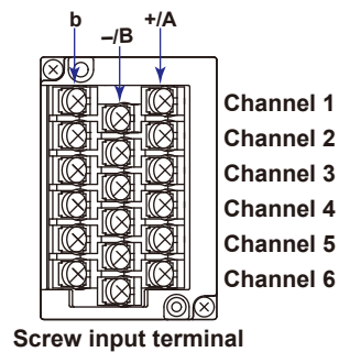
Screw input terminal
