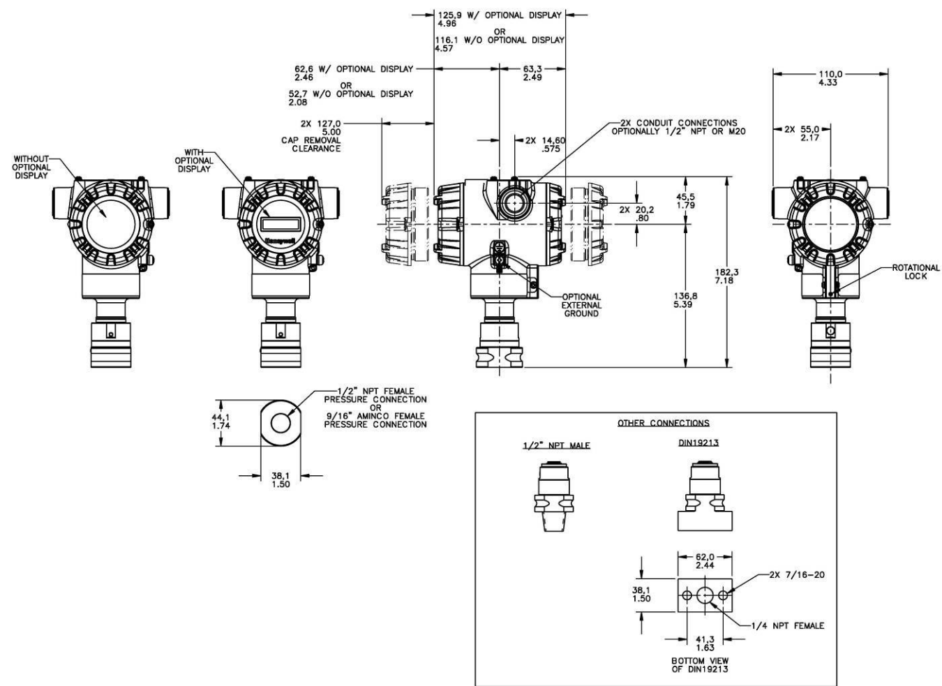
Figure 4– Typical mounting dimensions of STA72L, STA74L, & STA77L for reference
