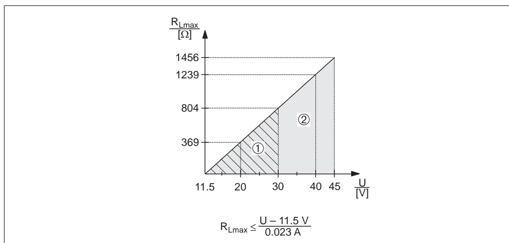
Load diagram
