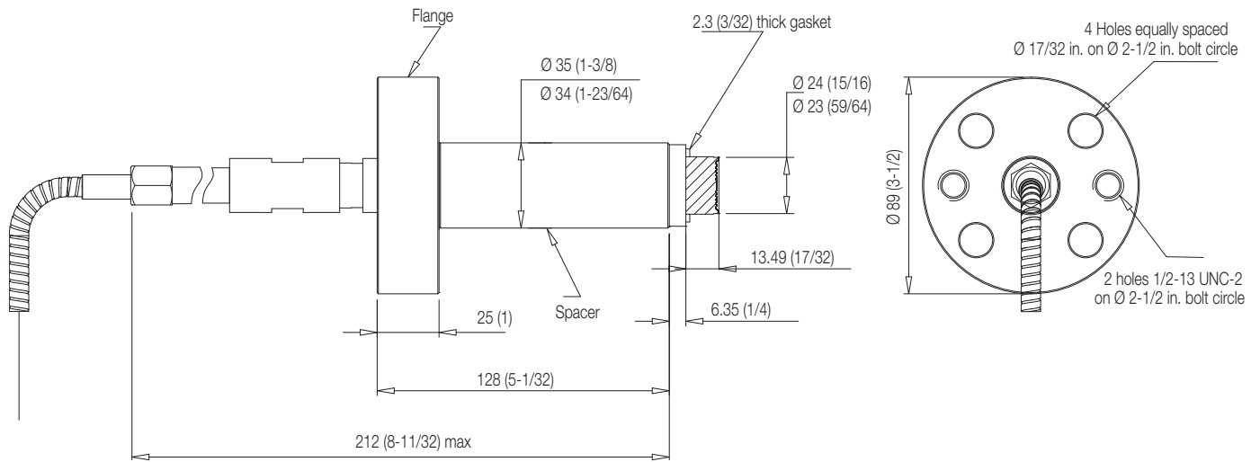
3 1/4 in. flange extended - type 91 modified
