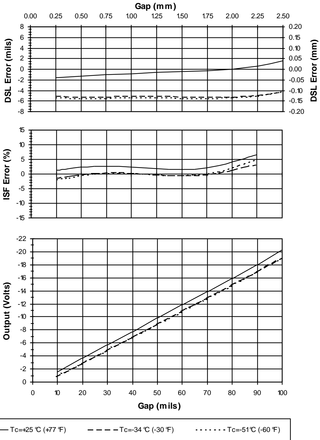
Figure 2: Typical 3300 XL 8mm 9 m Proximito Sensor with 8m of Extension Cable at T_c (Probe is at 25 °C)
