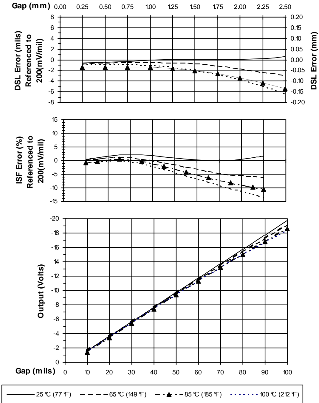
Figure 1: Typical 3300 XL 8 mm 5m Proximitor Sensor with 4m Extension Cable at T_h (Probe is at 25°C)
