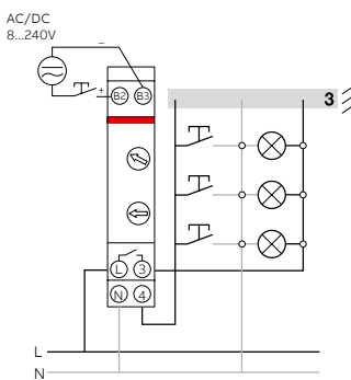
3-wire configuration E 232E-8/230Multi 10
