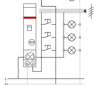
4-wire configuration E 232E-230N
