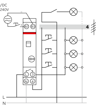
4-wire configuration E 232E-8/230N
