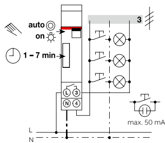
3-wire configuration E 232-230
