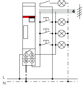
4-wire configuration E 232-230
