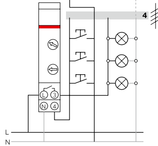
4-wire configuration E 232E-8/230N
